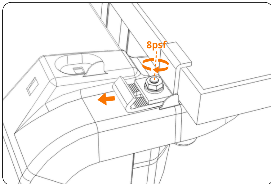
Fig. 9 Module Attachment
