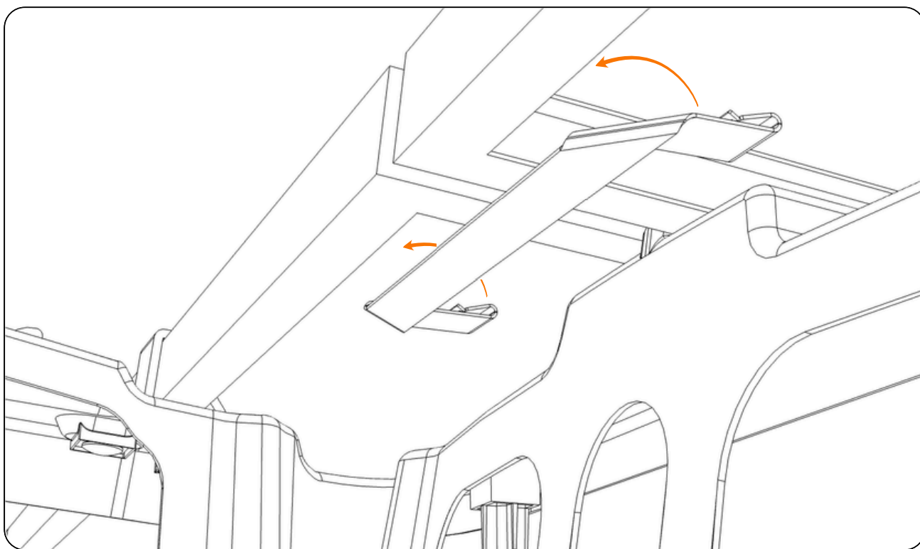
Fig. 17 FR-SBJ Installation
