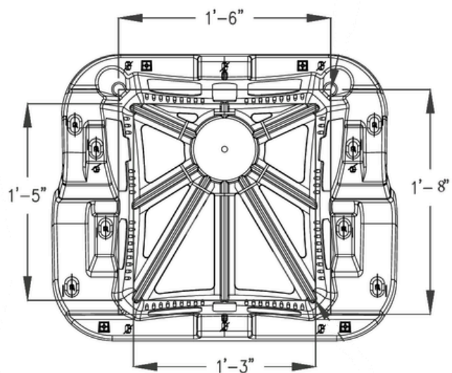
FR510-6-10dg 304/316
